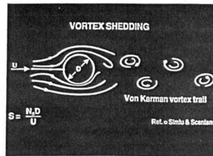
Figure 3.3: Vortex shedding.
