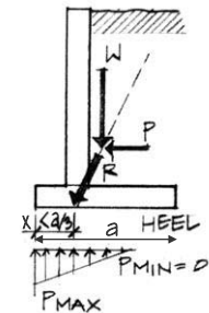
Figure 3.88 Tension possible at the heel.
