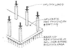
Figure 4.26 Mat or raft foundation.
