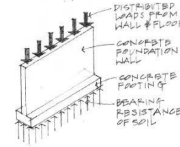
Figure 4.25 Wall footing.
