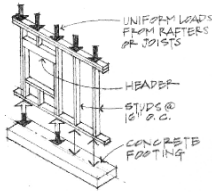
Figure 4.16 Stud wall with a window opening.
