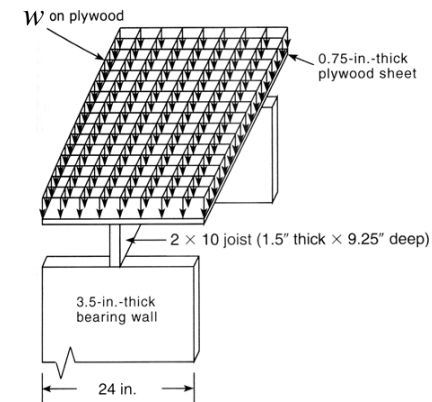
Figure 2.7 Area-distributed load (pressure) on floor decking.
