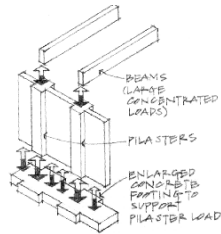
Figure 4.17 Pilasters supporting concentrated beam loads.
