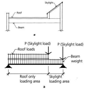
Figs. 1.1a, 1.1b Structural loading diagram of an architectural condition
