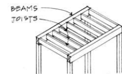
(b) Short joists loading relatively long beams yield shallow joists and deep beams. The individual structural bays are more clearly expressed.
