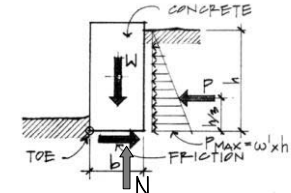
Figure 3.80 FBD of a gravity retaining wall.
