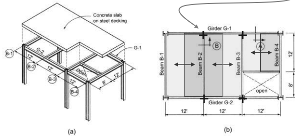
Figure 5.54 (a) Isometric view of partial steel framing arrangement. (b) Partial floor framing—office structure.
