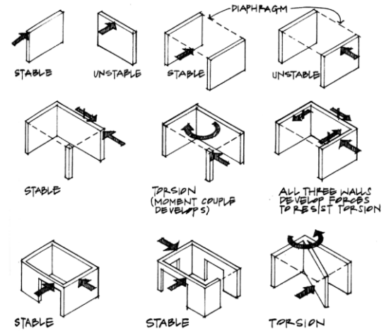
Figure 4.54 Various shearwall arrangements—some stable, others unstable.
