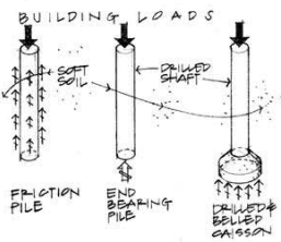
Figure 4.27 Pile foundations.
