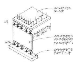
Figure 4.12 Uniform wall load from a slab.
