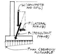
Figure 3.81 Bearing pressure under the wall footing.
